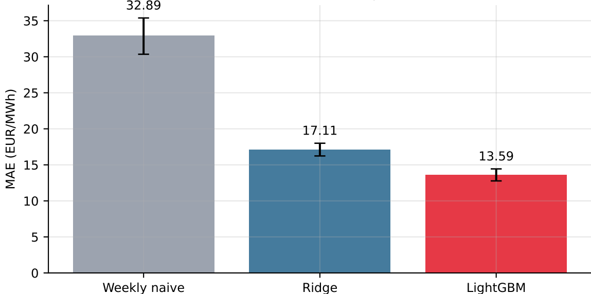
Full-year walk-forward error with day-block 95% intervals
